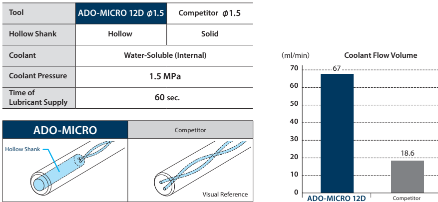
Figure 4. Relationship between shank structure and coolant flow volume
